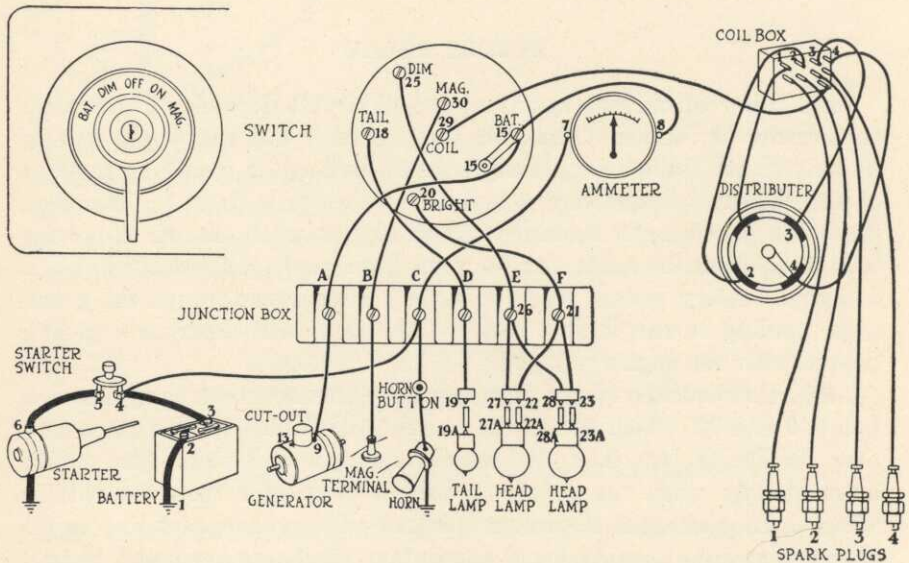
FIG. 87.—Standard Ford starting, lighting and ignition system.
