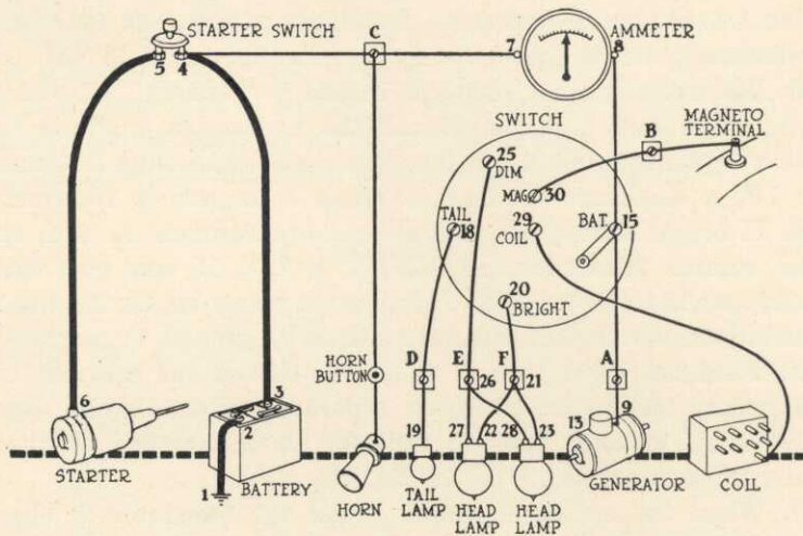
FIG. 86.—Standard Ford starting, lighting and ignition system arranged to illustrate the “parallel principle”—see Fig. 84.
