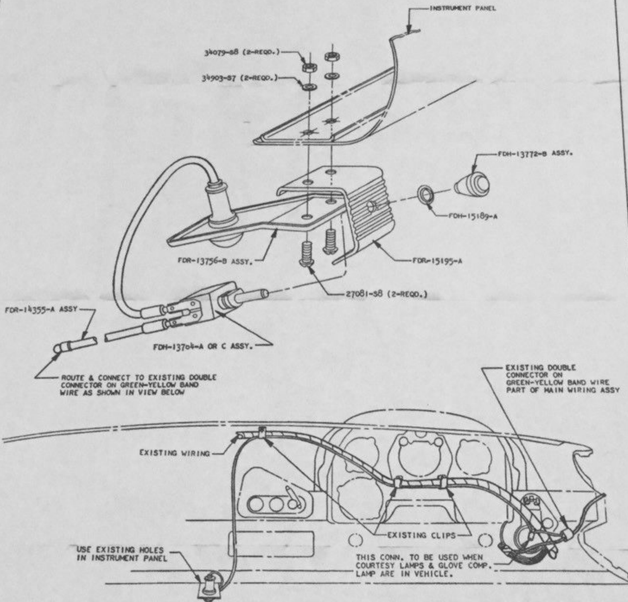
REAR VIEW OF INSTRUMENT PANEL
